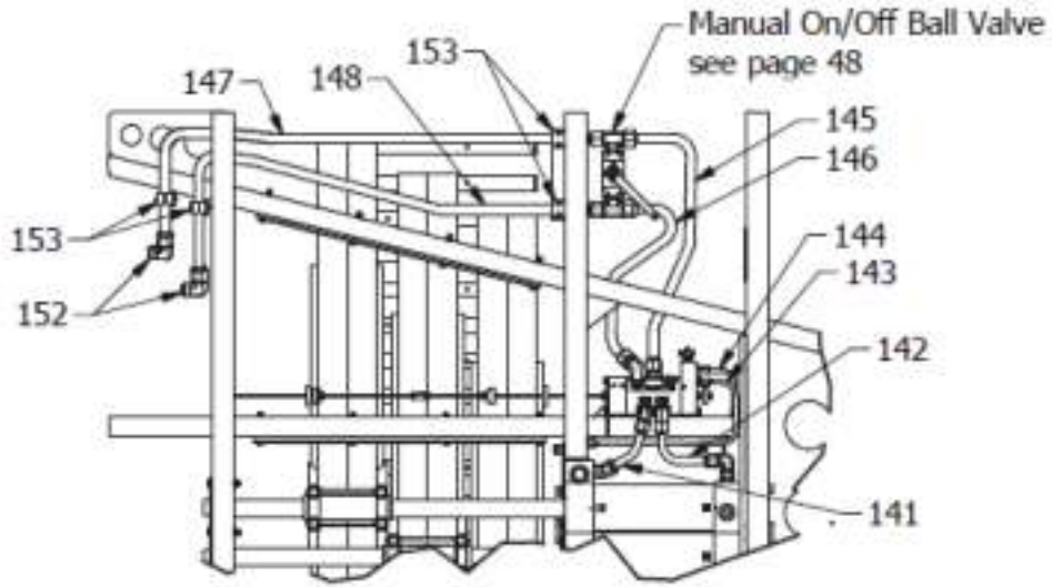
Manual Ball Valve Tube Set #139
