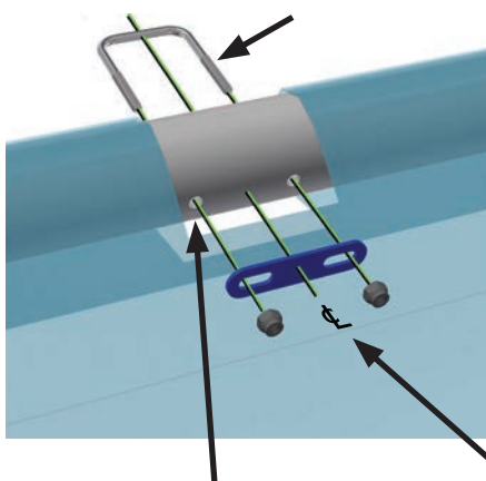
Drill (2) 3/8" [9.5 mm] holes through the top pipe for mounting the U-bolt
