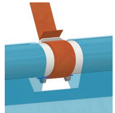
Wrap the end of the strap around the top pipe and secure it to the pipe using the U-bolt assembly.
