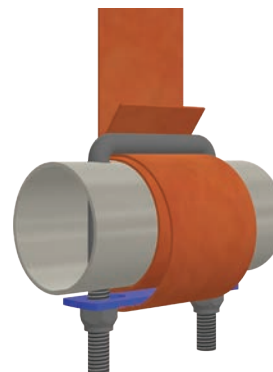
Wrap the end of the strap around the top pipe and secure it to the pipe using the U-bolt assembly.
